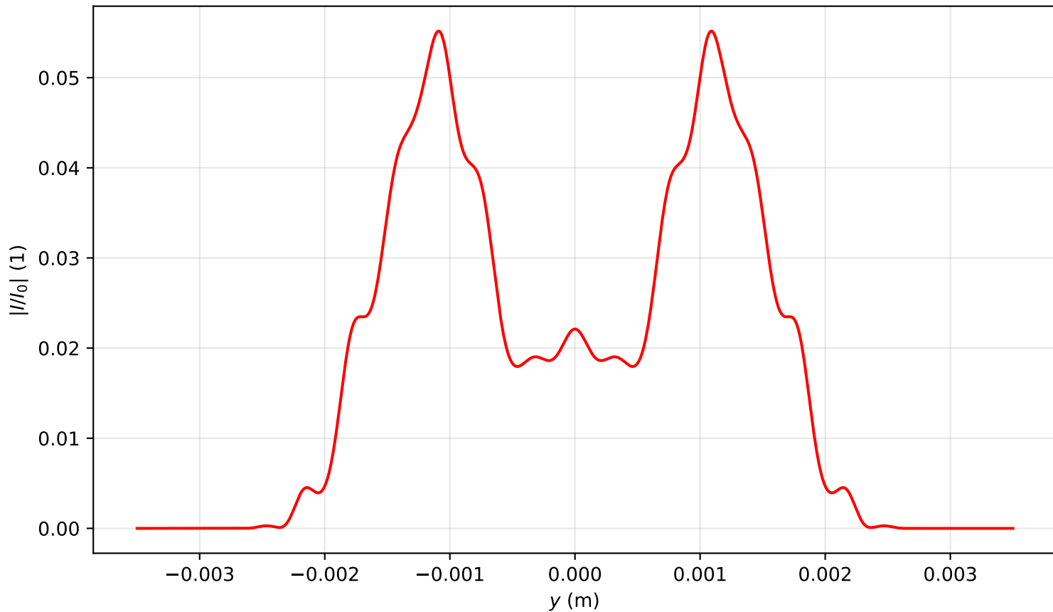
Intensity profile I(x=0, y, z=3.582)/I_0 , P_{in}=6.0P_{cr} , artificial time
